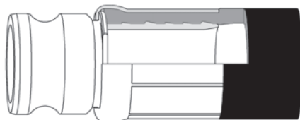
Crimped Assembly
