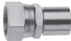
female JIC swivel (crimp collar included)
