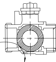
Valve - closed and draining occurs. Upstream seat prevents air flow. Downstream system is vented to atmosphere.
