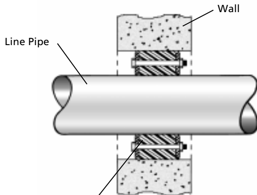
PEN-SEAL Wall Penetration Seal by PROCO PRODUCTS, INC.
