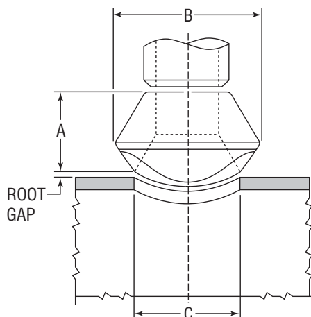
BUTTWELD Standard
