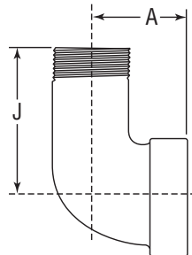
FIGURE 1170 90° Street Elbow
