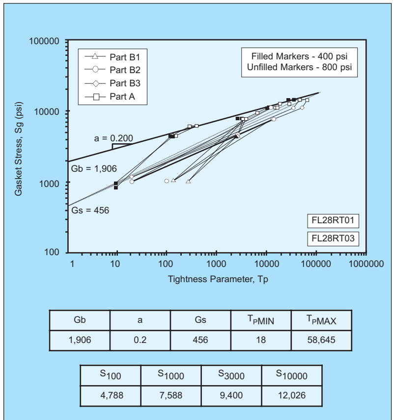
Room Temperature Tightness (ROTT) behavior characterization (Refer to page 41 for new method for determining factors.)
