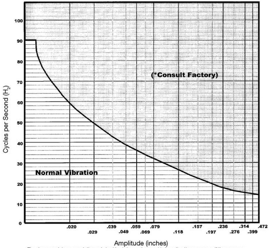
The above graph is representative and should only be used as a guide for estimation purposes. If there are any questions, or your application is near the "Consult Factory" region, please contact Hose Master Inside Sales.
