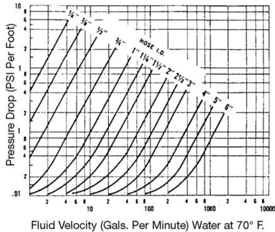
Pressure Drop Graph for Water
