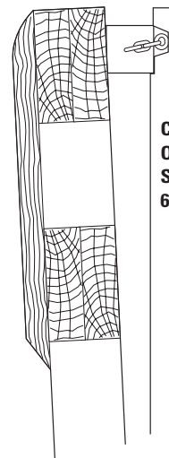
CROSS SECTION OF DOCK FRONTAL SYSTEM WITH 700 SERIES FENDER
