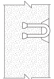
CROSS SECTION OF RECESSED "EYE RING" EMBEDDED IN CONCRETE
