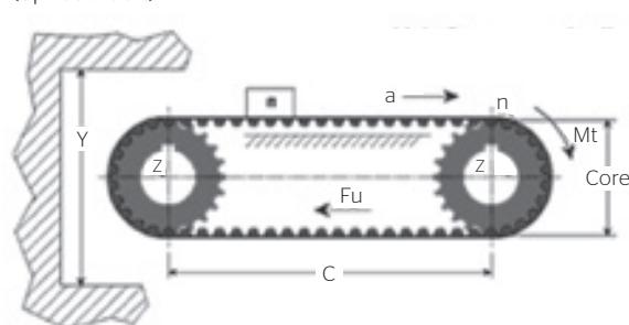
Linear Conveyance Application (Spliced belt)
