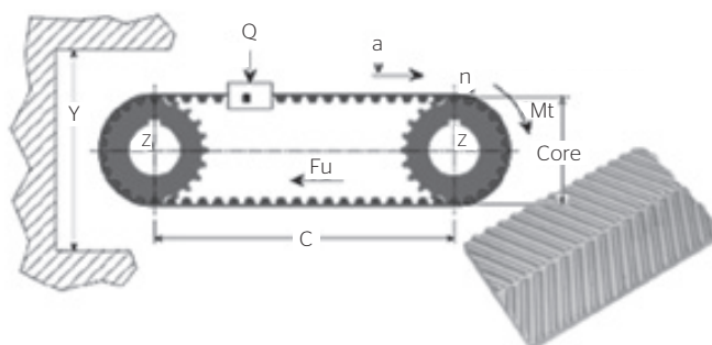
Linear Motion Drive (Open End Pd® belt)
