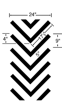
3/4" High x 1 1/4" Wide Cleats for 24" or Wider Belts
