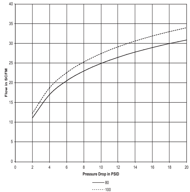
Twist-lock (1/4")
