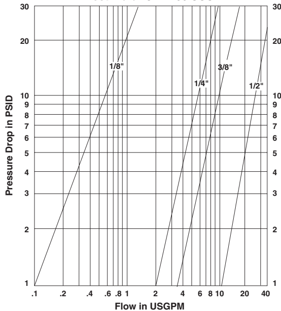
ST Series (1/8; 1/4; 3/8; 1/2") Test Fluid: Oil - 200 SUS
