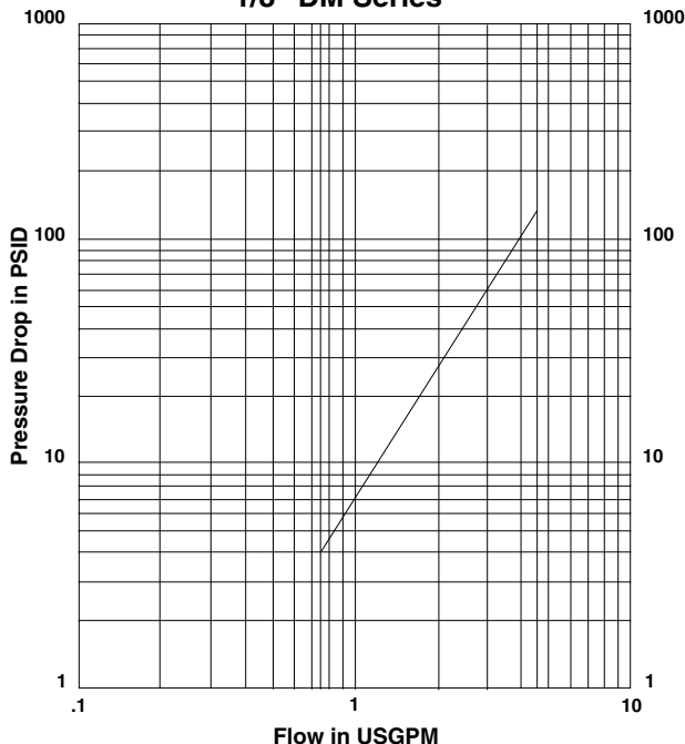
Water Pressure Drop 1/8" DM Series
