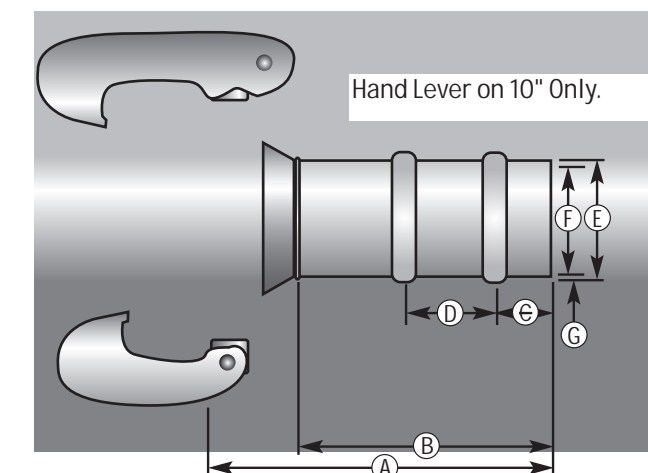
10" Female Hose Tail
